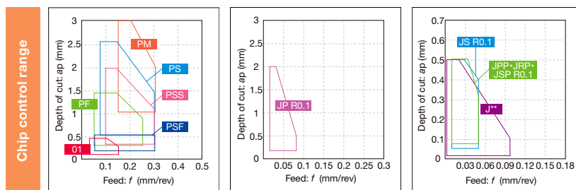
*Chip control range with typical R0.1
