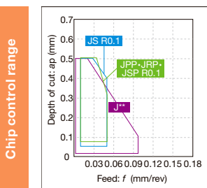
*Chip control range with typical R0.1
